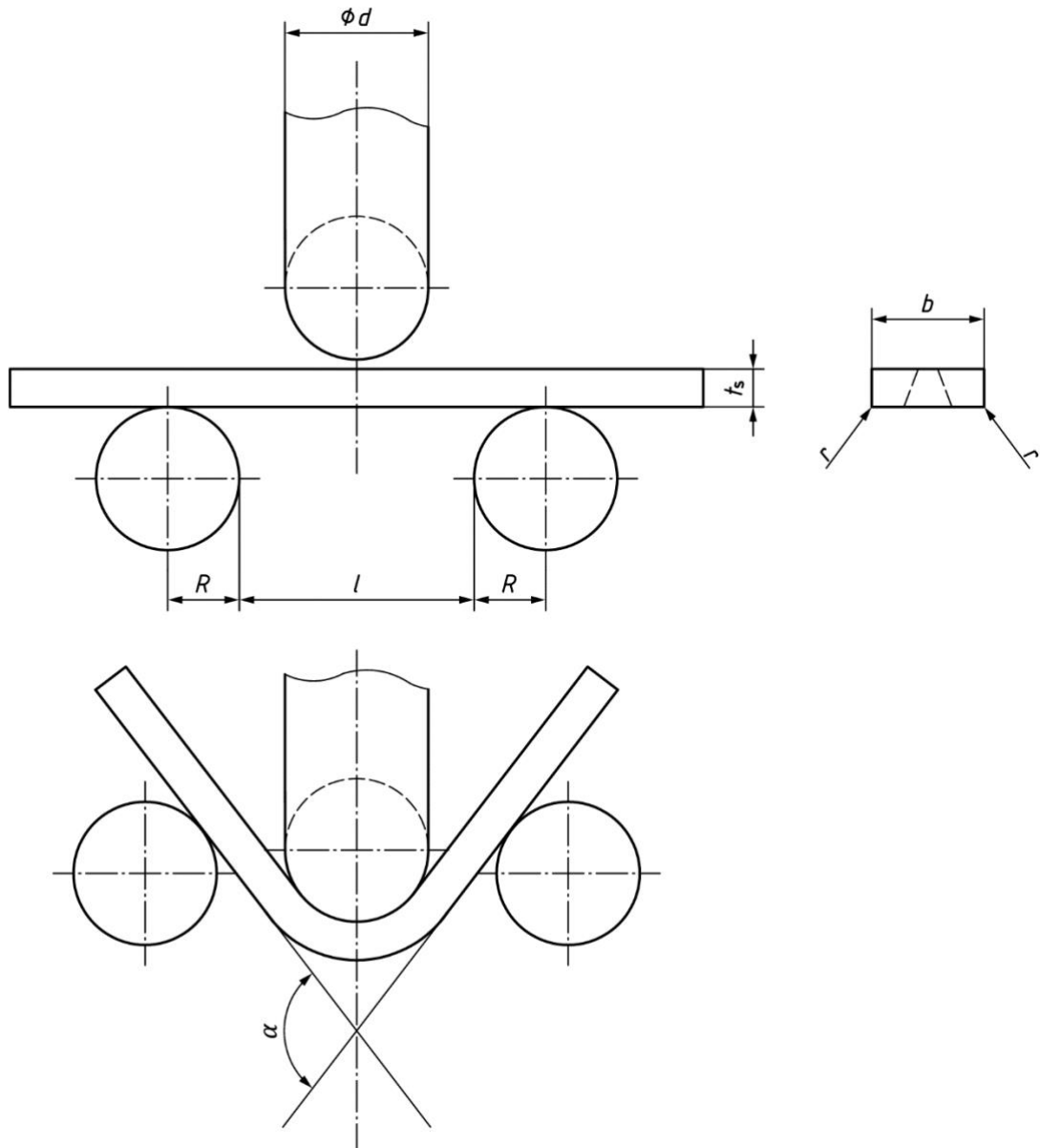
Figure 13 — Longitudinal bend test
