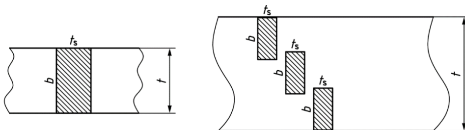
Figure 9— Root and face bend test specimens for a butt weld (TFBB, TRBB, LFBB, LRBB and FBCB)
