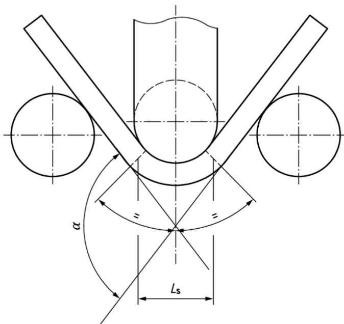
Figure 12 — Transverse side bend test
