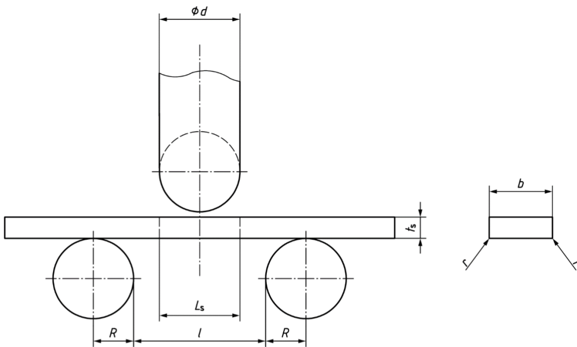
Figure 11 — Transverse face or root bend test
